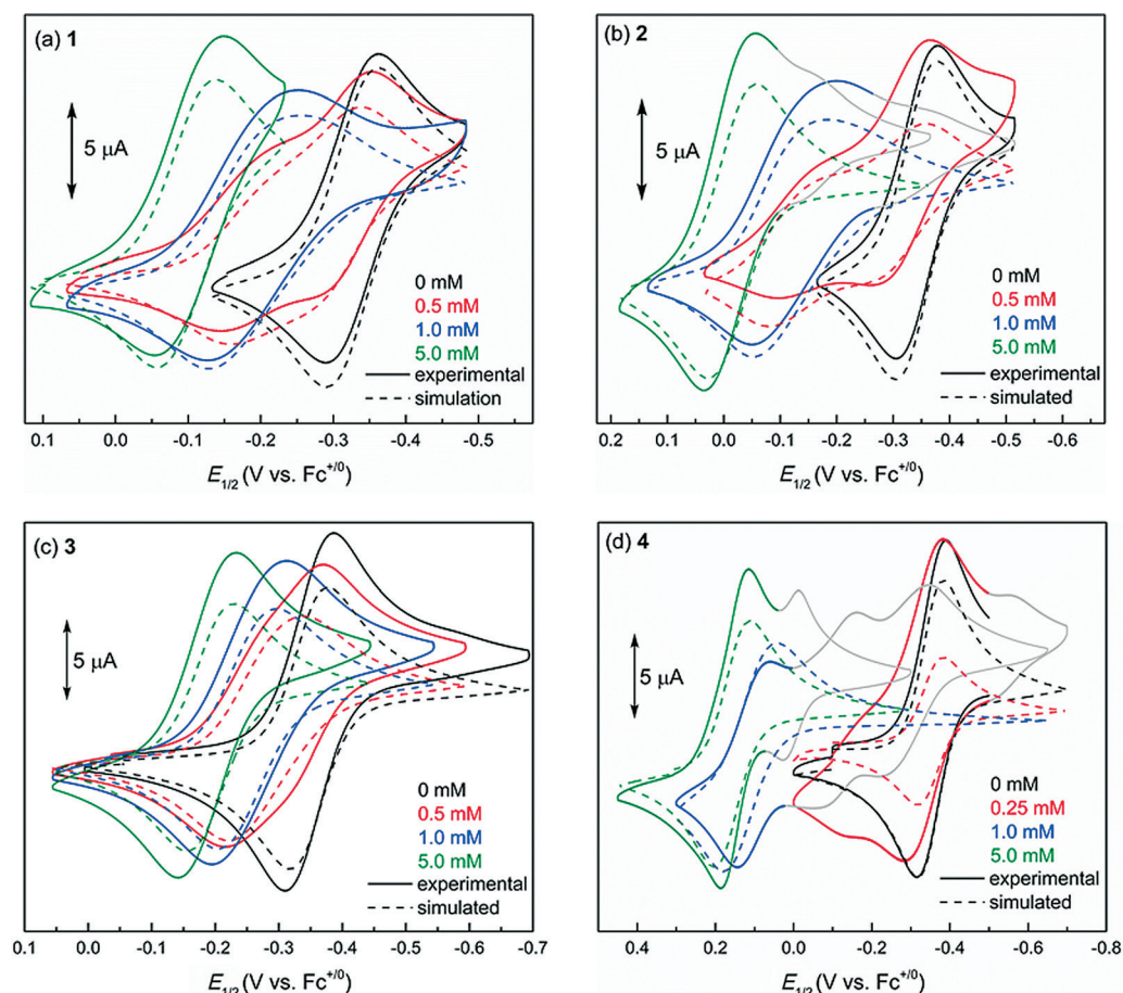
Figure 3. Experimental CV data and comparison with simulation. CVs (0.1 Vs -1 ) recorded for 0.5 mM Q in 0.1 M nBu 4 NBArF 74 /CH 2 Cl 2 (glovebox) in the presence of increasing concentrations of a) 1 , b) 2 , c) 3 , and d) 4 .
