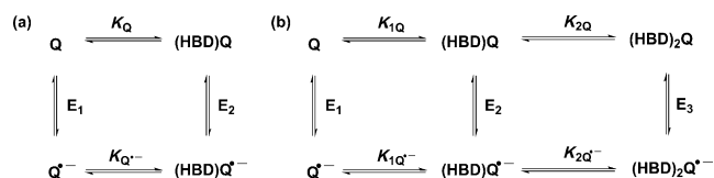
Scheme 1. a) Square scheme describing pathways for HBD-coupled ET to quinones and their associated equilibrium constants. b) Extended square scheme accounting for two binding events.
